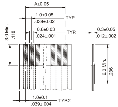
Accommodated FFC
